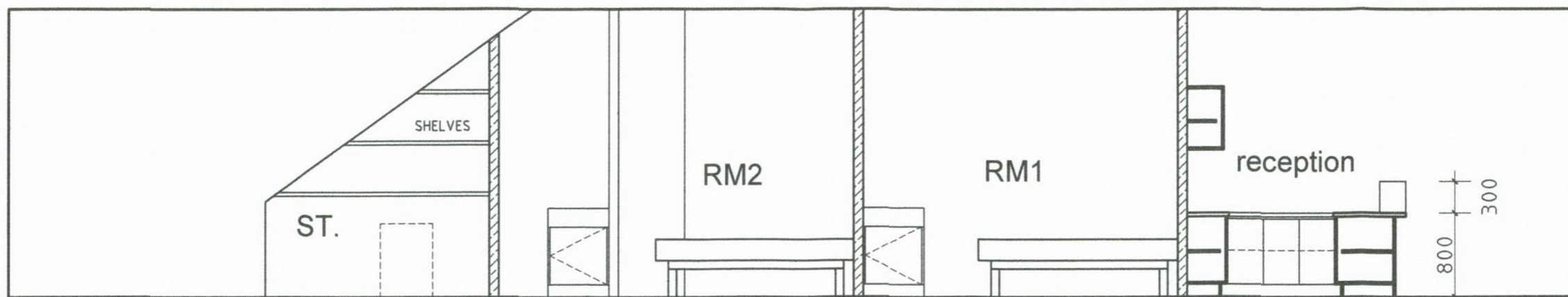
1 ELEVATION scale 1:50
