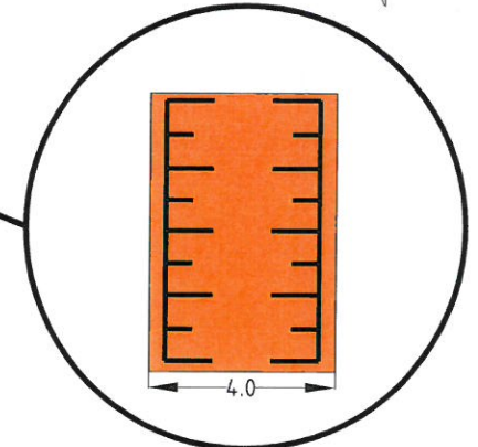
TYPICAL SPEED HUMP DETAILS
