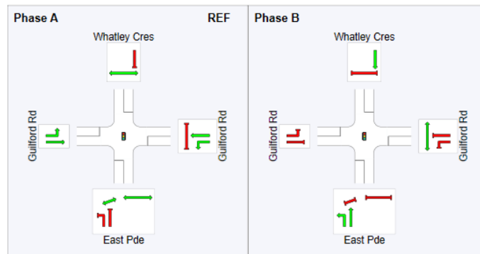
Figure 2: Existing layout and phasing from SIDRA
