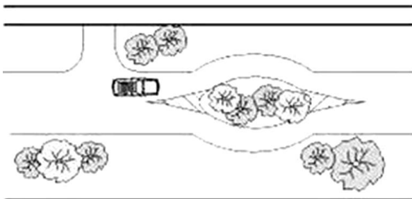
Blister islands on narrow carriageways may require widening
